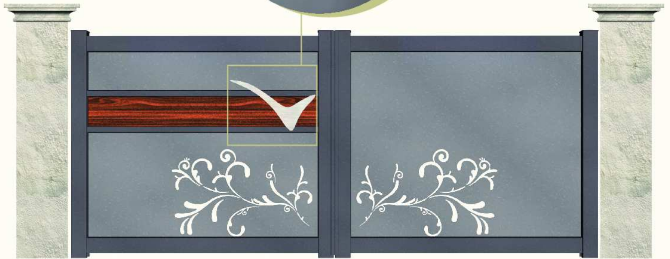
Andromeda
