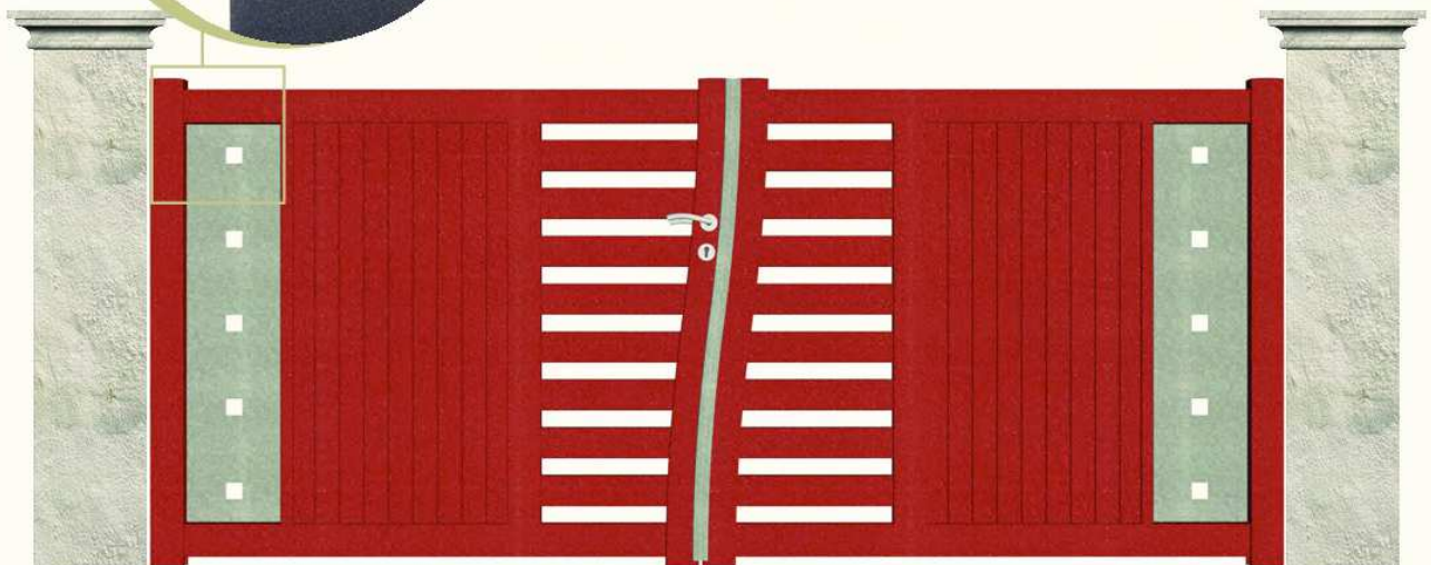
Sculptor
