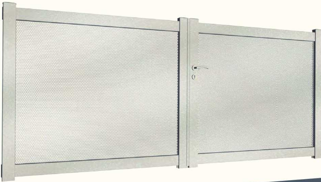
Tucana A
